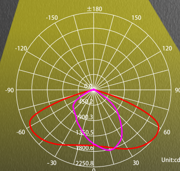
C plane lighting distributions
