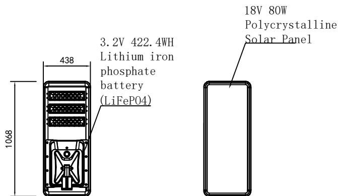
Integrated detailed drawing
