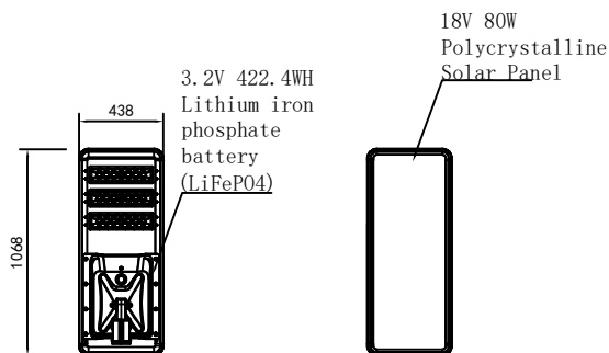
Integrated detailed drawing
