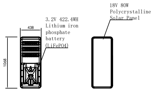
Integrated detailed drawing
